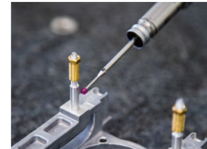
Bracket measurement
