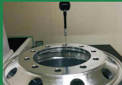
Wheel measurement
