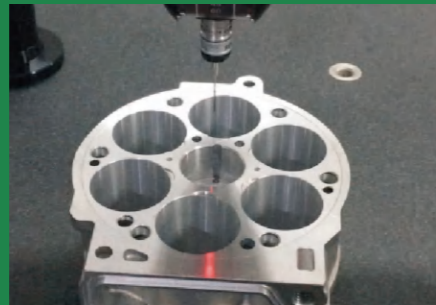
Cylinder measurement
